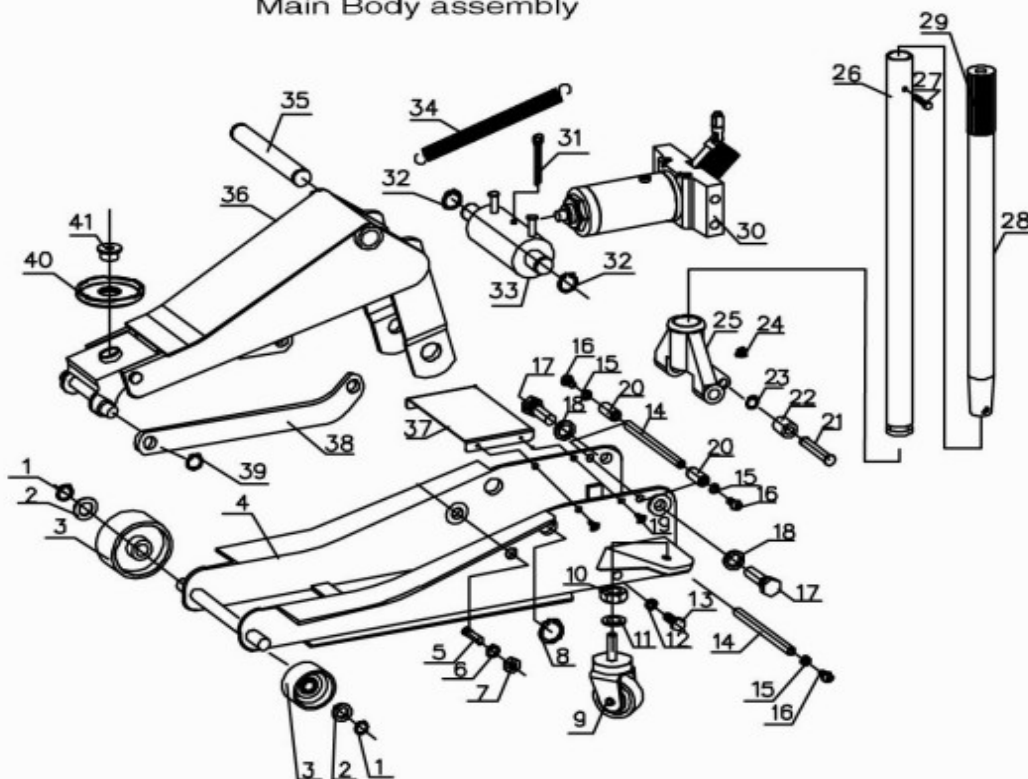
Main Body assembly
